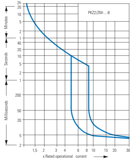
Tripping characteristic curves, line protection
