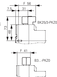
BK25/3-PKZ0
