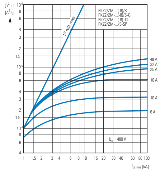
Let-through characteristics, high-capacity compact starters and circuit-breakers + current limiters CL
