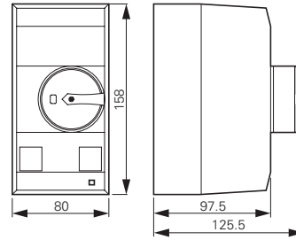
CI-PKZ10G...M
