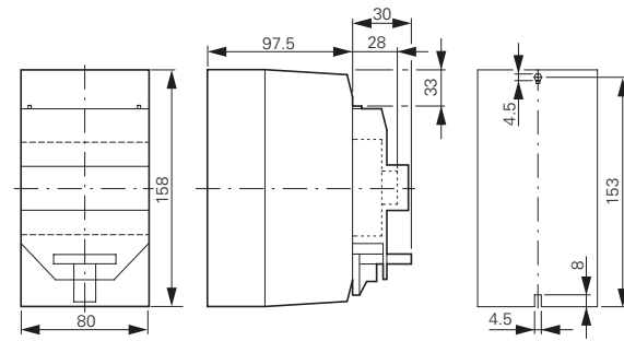
CI-PKZ0...M
