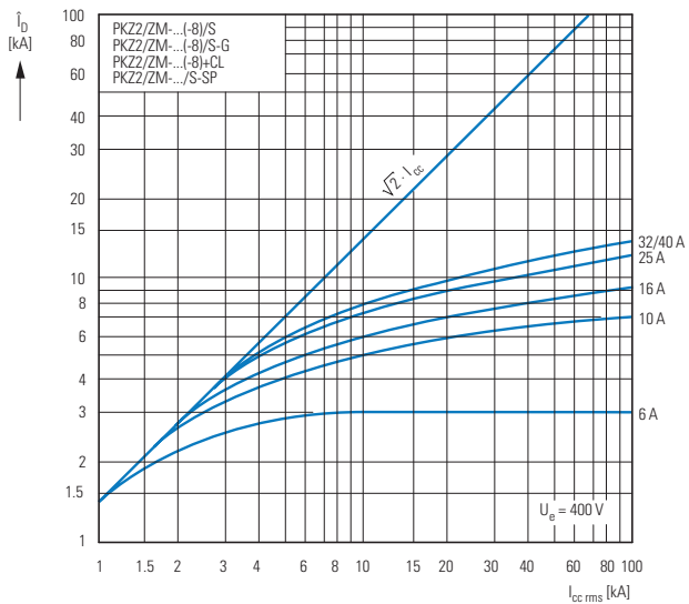
Let-through characteristics, high-capacity compact starters and circuit-breakers + current limiters CL
