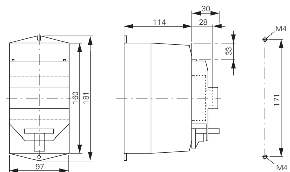
CI-K2-PKZ0...
