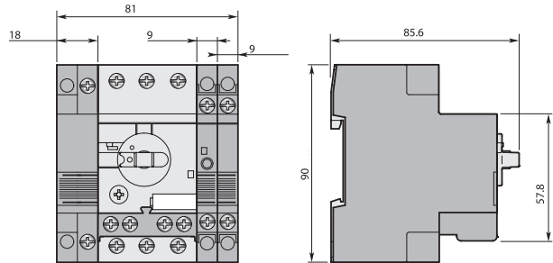
MS116 + UA1, AA1, SK1, HK1, CK1, HKF1-11
