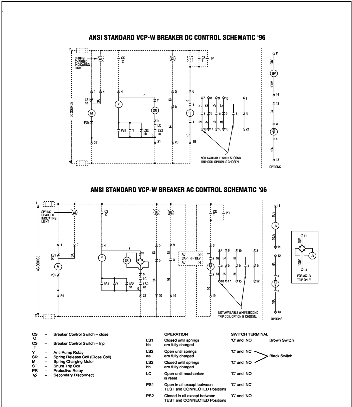
Figure 5-5 Typical VCP-W DC and AC Control Schemes
