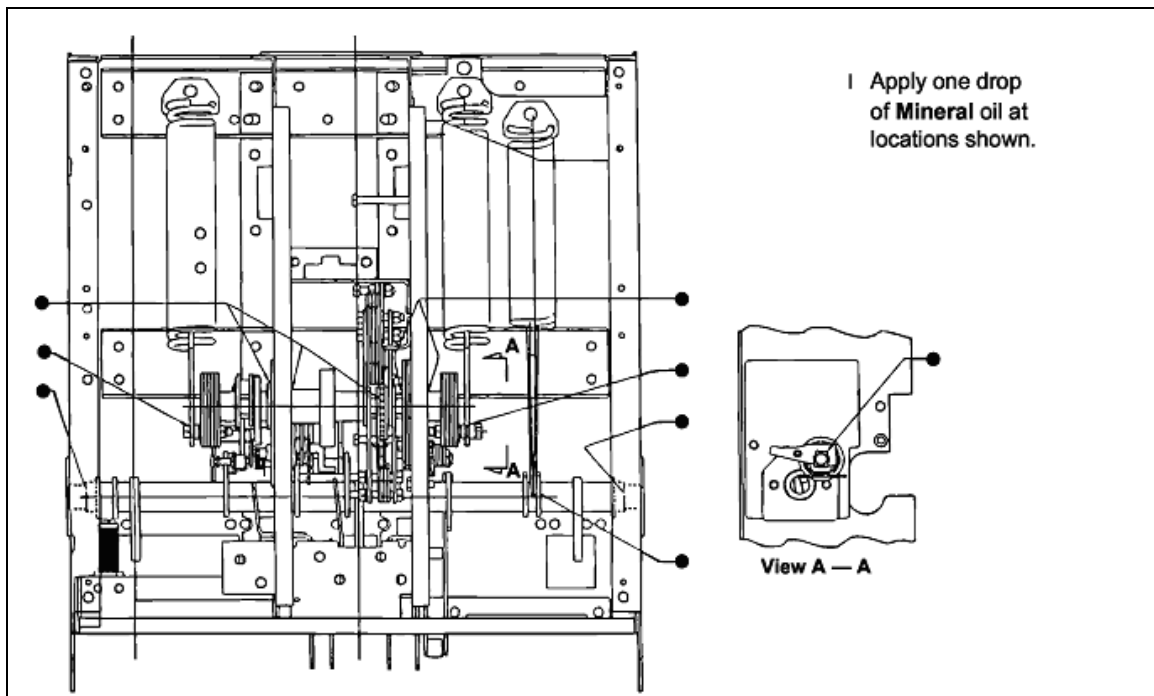
Figure 6-1 lubrication points
